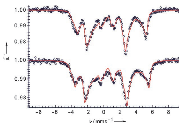
Figure 4. Applied field Mössbauer spectra of [\text{Fe}^{\text{III}}\text{L}_3] at 4.2 K with fields of 5 (bottom) and 7 T (top) applied perpendicular to the \gamma -beam. The solid (red) lines are fitted Lorentzian line shapes.
